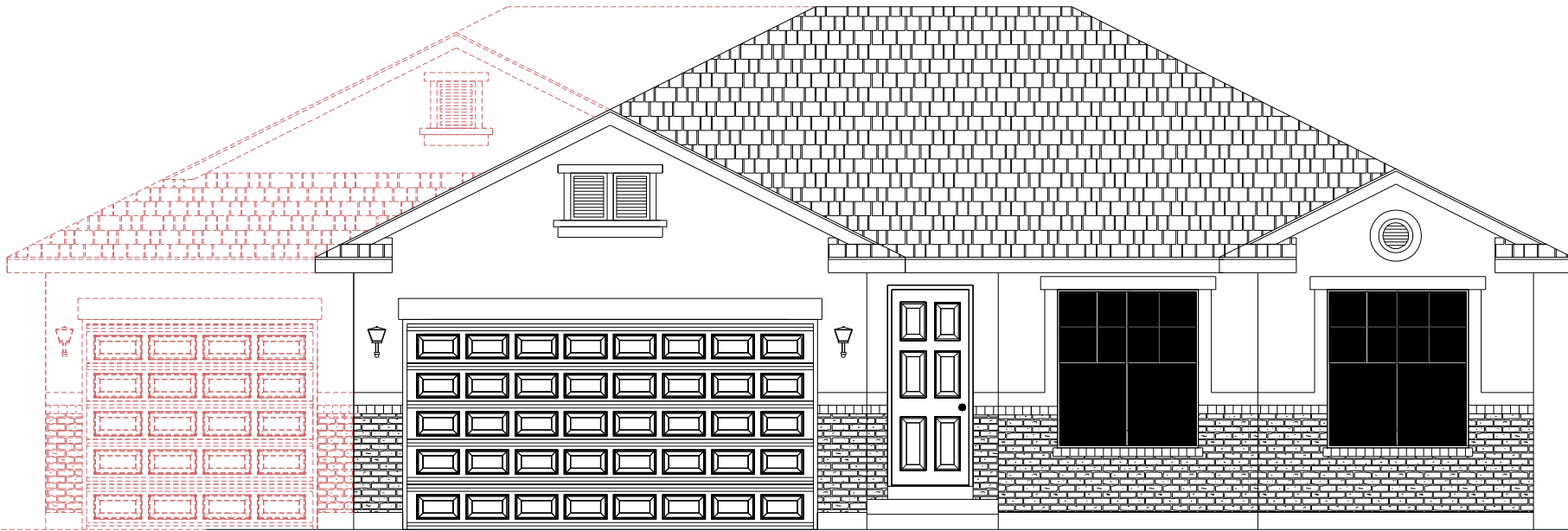
ELEVATION "A"
